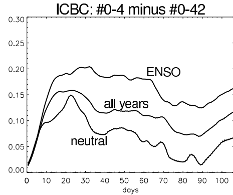
Fig. 13. Difference in global instantaneous skill of ICBC between large scale filtered and unfiltered data for ENSO years, all years (1980–2000), and neutral years.
