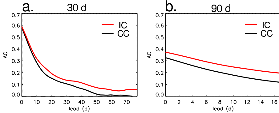
Fig. 4. Lag evolution of global 500hPa AC for simulation IC (red) and CC (black), verified against itself under the perfect model assumption. The curves show composite ensemble mean skill over 21 winter seasons (1980–2000): (a) from 30 days time averaged data; (b) from 90 days time averaged data.
