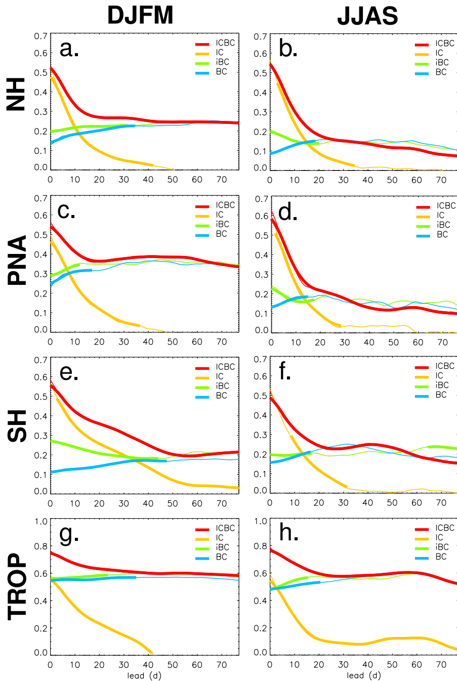
Fig. 7. Lag evolution of the spatial AC averaged over all years (1980–2000) from 30 days time averaged data. Panels (a)–(b) show the AC over the Northern Hemisphere ( 20^{\circ}\text{N} – 90^{\circ}\text{N} ), (c)–(d) for the PNA region ( 180^{\circ}\text{W} – 60^{\circ}\text{W} , 15^{\circ}\text{N} – 70^{\circ}\text{N} ), (e)–(f) for the Southern Hemisphere ( 20^{\circ}\text{S} – 90^{\circ}\text{S} ), and (g)–(h) for the tropics ( 20^{\circ}\text{M} – 20^{\circ}\text{S} ). The AC has been calculated from the 500 hPa surface except for the tropics, where the 200 hPa surface has been used. Left panels are from 15 December to 31 March, and right panels are from 15 June to 31 September. All experiments were verified against ICBC under the perfect model assumption.
