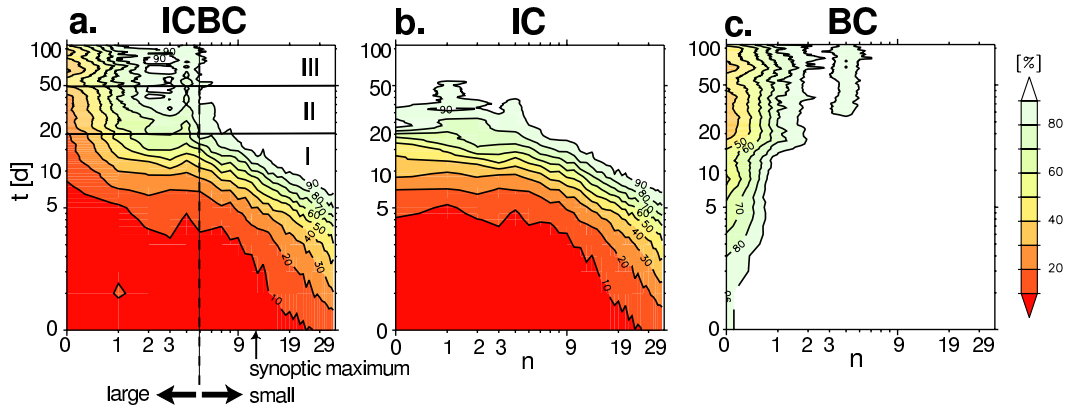
Fig. 11. Error energy spectrum as a function of total wavenumber n and lead time t for simulation ICBC (a), IC (b) and BC (c). 500hPa height ensemble mean fields of each simulation were verified against individual members of ICBC. Error energy is expressed in percent of the maximum saturation error.
