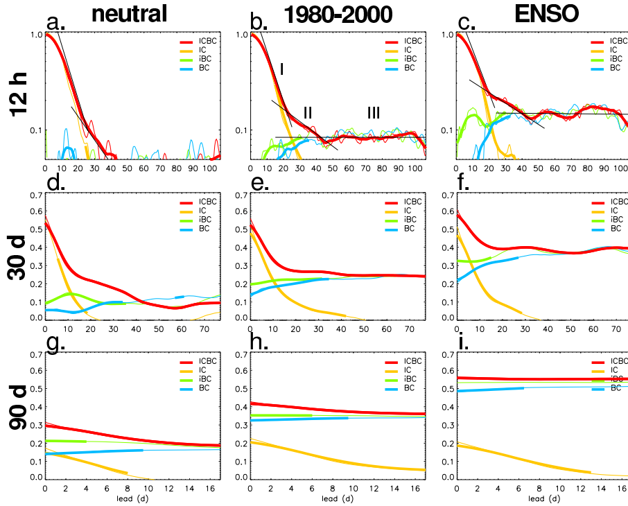
Fig. 6. Lag evolution of the spatial AC of the 500 hPa surface over the Northern Hemisphere ( 20^{\circ} N– 90^{\circ} N) from 15 December to 31 March. All experiments have been verified against experiment ICBC. Results are based on all ensemble members of the indicated years. Top panels show AC from unaveraged 12 h data, middle panels are from 30 days time averaged data, and bottom panels are from 90 days time averages. Thick lines have been smoothed with a 10-day running mean filter, and are only shown where the AC is significantly (5% error) different from zero and from the reference experiment ICBC. Y-axis denotes the AC. Note the logarithmic y-axis for the top panels (range: 0.05–1.0).
