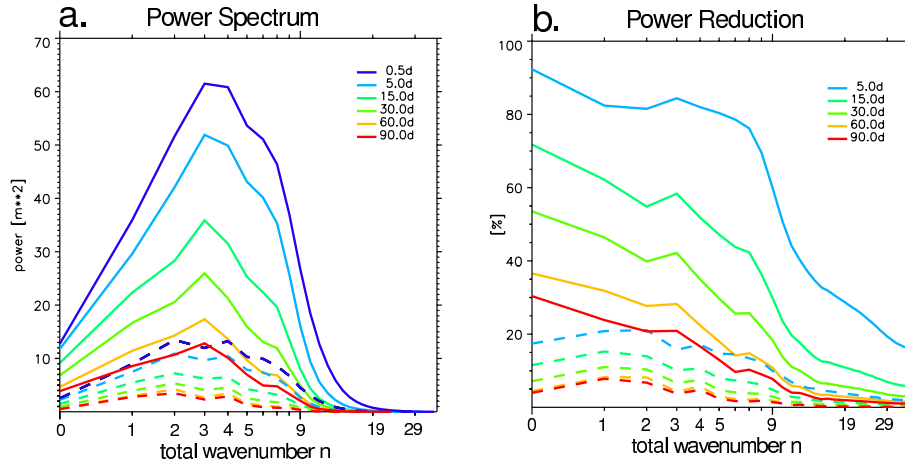
Fig. 2. (a) Wavenumber spectra derived from the 500hPa fields of simulation CC for various temporal averaging intervals. Dashed lines show spectra for ensemble and time averaged data. (b) Power reduction relative to unaveraged spectrum without (continuous) and with (dashed) ensemble averaging. Note logarithmic scale for x-axis.
