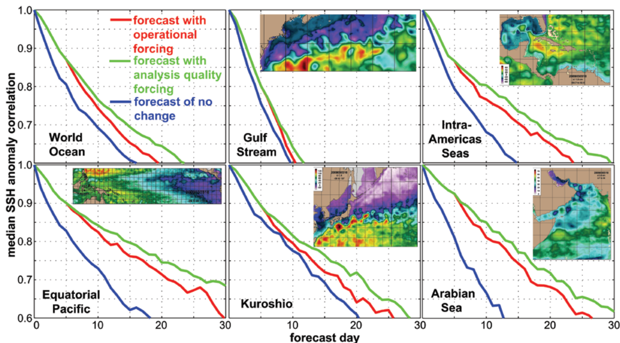
Figure 5: Verification of 30-day ocean forecasts: median SSH anomaly correlation vs. forecast length in comparison with the verifying analysis for the global U.S Navy HYCOM over the world ocean and five subregions. The red curves verify forecasts using operational atmospheric forcing, which reverts toward climatology after five days. The green curves verify “forecasts” with analysis quality forcing for the duration and the blue curves verify forecasts of persistence (i.e., no change from the initial state). The plots show median statistics over twenty 30-day HYCOM forecasts initialized during January 2004 - December 2005, a period when data from three nadir-beam altimeters, Envisat, GFO and Jason-1, were assimilated. The reader is referred to Hurlburt et al. (2008, 2009) for a more detailed discussion of these results. From Chassignet et al. (2009).
