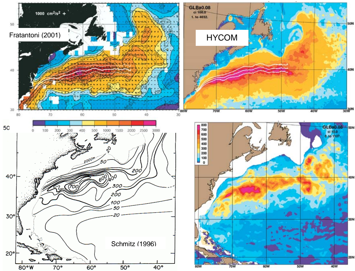
Figure 6: Surface (top panels) and 700 m (lower panels) eddy kinetic energy from observations (left panels) and HYCOM over the period 2004–2006 (right panels). The observed surface eddy kinetic energy (upper left panel) is from Fratantoni (2001) and the 700 m eddy kinetic energy (lower left panel) is from Schmitz (1996). The units are in \text{cm}^2/\text{s}^2 . Overlaid on the top panels is the Gulf Stream north wall position \pm 1 standard deviation. From Chassignet et al. (2009).
