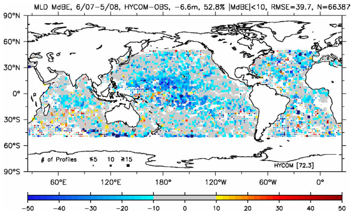
Figure 8: Median bias error (in meters) of mixed layer depth (MLD) calculated from simulated and approximately 66000 unassimilated observed profiles over the period June 2007-May 2008. Blue (red) indicates a simulated MLD shallower (deeper) than observed; 53% of the simulated MLDs are within 10 m of the observation and these are represented as gray. The basin-wide median bias error is -6.6 meters and the RMS error is 40 meters. From Chassignet et al. (2009).
