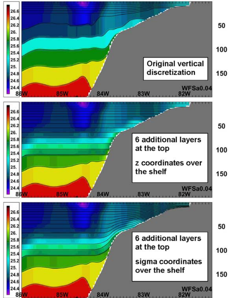
Figure 3: Cross-sections of layer density and model interfaces across the West Florida Shelf in a 1/25^\circ West Florida Shelf subdomain covering the Gulf of Mexico east of 87^\circ\text{W} and north of 23^\circ\text{N} (Halliwell et al., 2009). From Chassignet et al. (2006, 2007).
