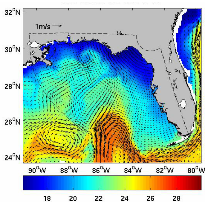
Figure 9: Sea surface temperature ( ^{\circ}\text{C} ) and surface velocity fields from the ROMS West Florida Shelf domain (inside the dashed lines) and the HYCOM ocean prediction system (outside the dashed lines). From Chassignet et al. (2009).
