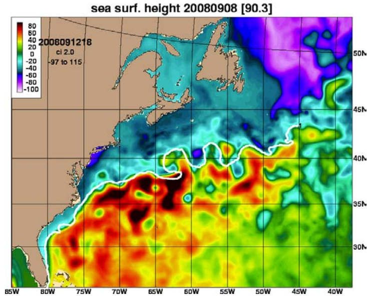
Figure 7: Modeled analysis of the sea surface height field on September 8, 2008. The white line represents the independent frontal analysis of sea surface temperature observations performed by the Naval Oceanographic Office. From Chassignet et al. (2009).
