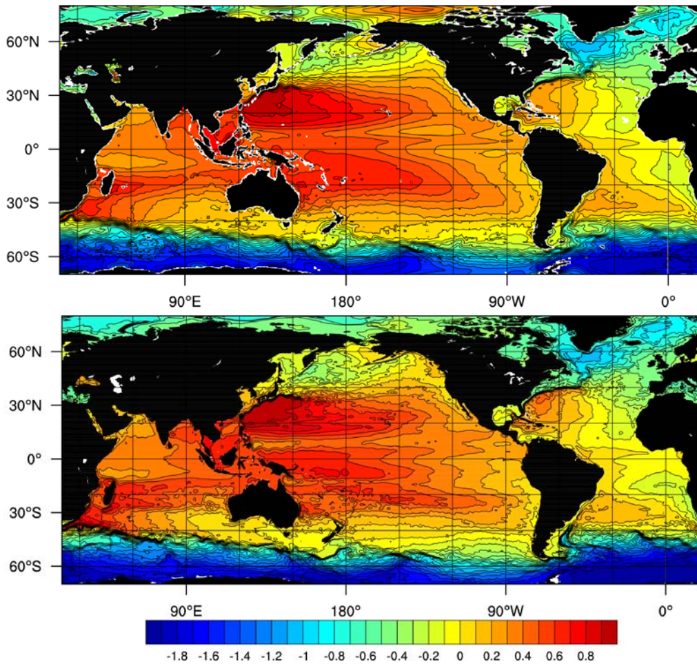
Figure 4: Mean SSH (in cm) derived from surface drifters (Maximenko and Niiler, 2005) (top panel) and from a non-data assimilative HYCOM run corrected in the Gulf Stream and Kuroshio regions using a rubber-sheeting technique (bottom panel). The RMS difference between the two fields is 9.2 cm. From Chassignet et al. (2009).
