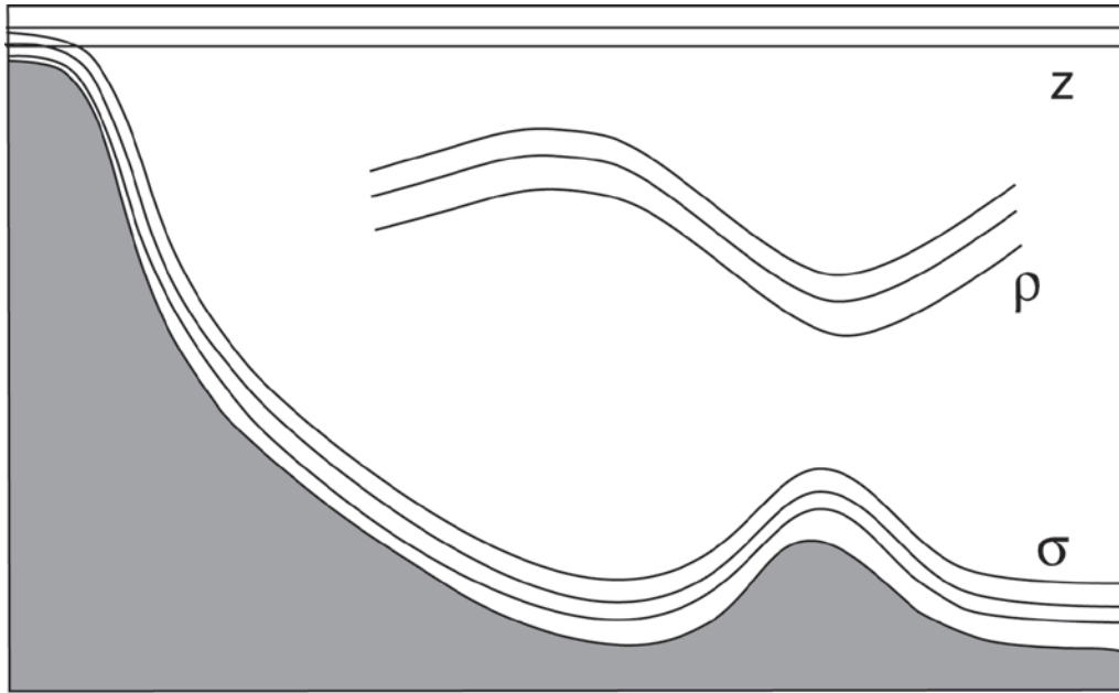
Figure 1: Schematic of an ocean basin illustrating the three regimes of the ocean germane to the considerations of an appropriate vertical coordinate. The surface mixed layer is naturally represented using fixed depth z (or pressure p ) coordinates, the interior is naturally represented using isopycnic \rho_{\text{pot}} (potential density tracking) coordinates, and the bottom boundary is naturally represented using terrain-following \sigma coordinates. Adapted from Griffies et al. (2000a).
