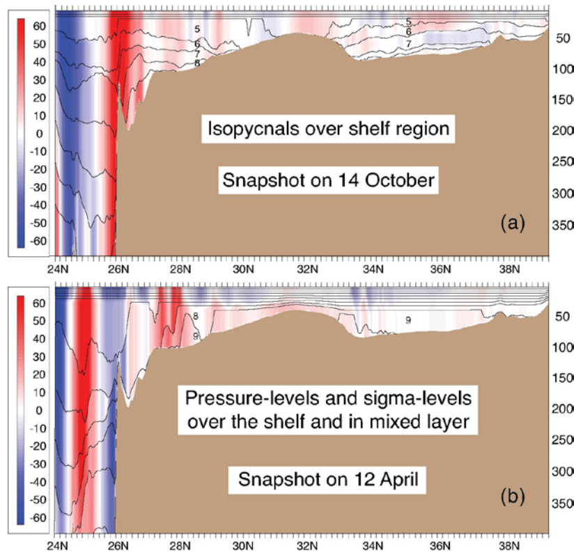
Figure 2: Upper 400 meters north-south velocity cross-section along 124.5°E in a 1/25° East China and Yellow Seas HYCOM embedded in a 1/6° North Pacific configuration forced with climatological monthly winds: (a) In the fall, the water column is stratified over the shelf and can be represented with isopycnals ( \rho_{pot} ); (b) In the spring, the water column is homogenized over the shelf and the vertical coordinate becomes a mixture of pressure ( p ) levels and terrain-following ( \sigma ) levels. The isopycnic layers are numbered over the shelf; the higher the number, the denser the layer. From Chassignet et al. (2007).
