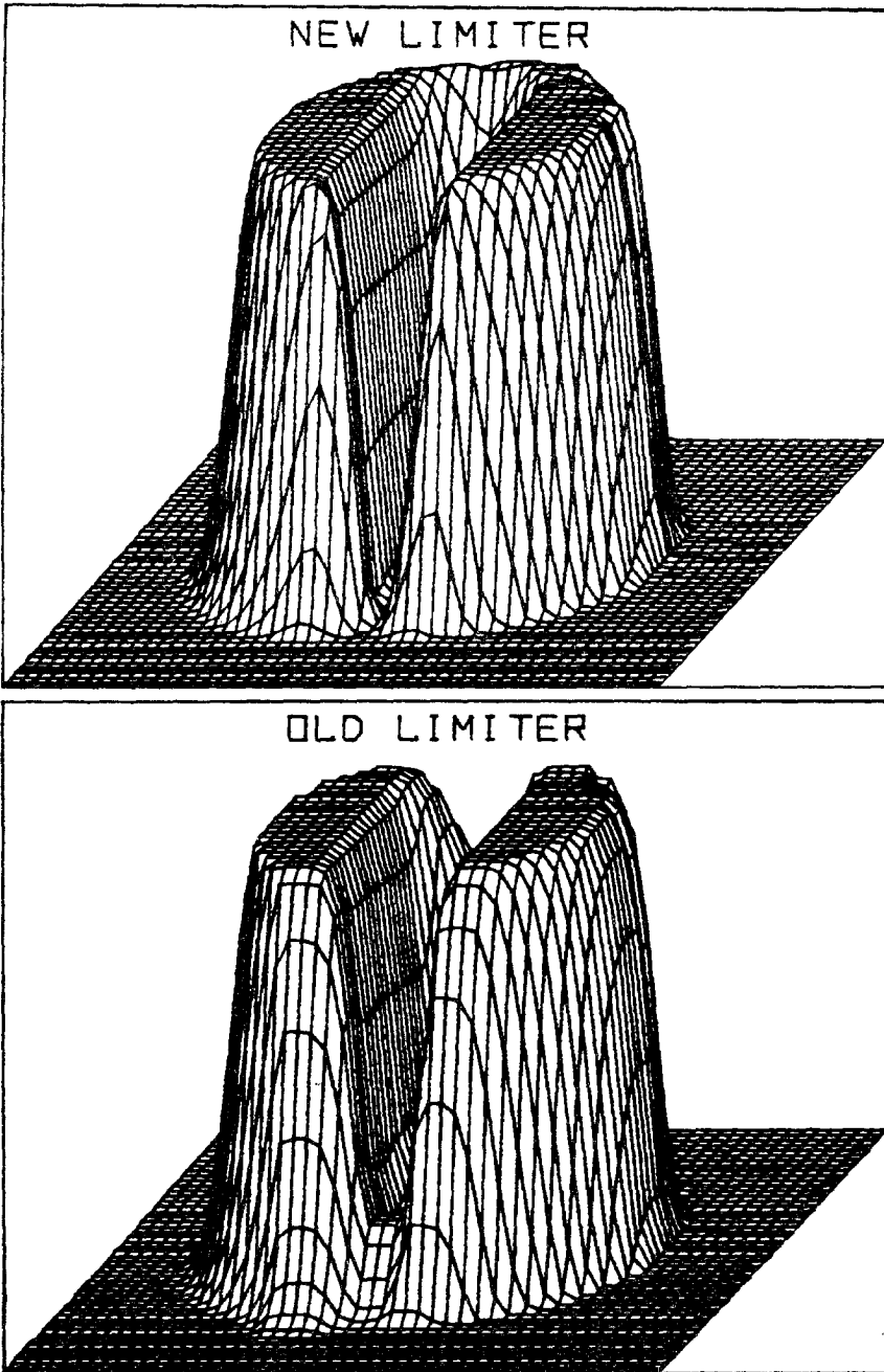
FIG. 13. Comparison of perspective views of the w profile after 157 iterations ( \frac{1}{4} revolution) with both the old and new flux limiters. The perspective view has been rotated with the cylinder, so that direct comparison with Fig. 12 can be made. Again we plot only the 50 \times 50 grid centered on the analytic center of the cylinder. Features to compare are the filling-in of the gap, erosion of the "bridge," and the relative sharpness of the profiles defining the front surface of the cylinder.
