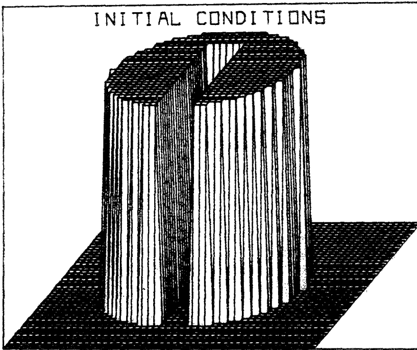
FIG. 12. Perspective view of initial conditions for the two dimensional solid body rotation problem. Note that only a 50 \times 50 portion of the mesh centered on the cylinder is displayed. Grid points inside the cylinder have w_{i,j} = 3.0 . All others have w_{i,j} = 1.0 .
