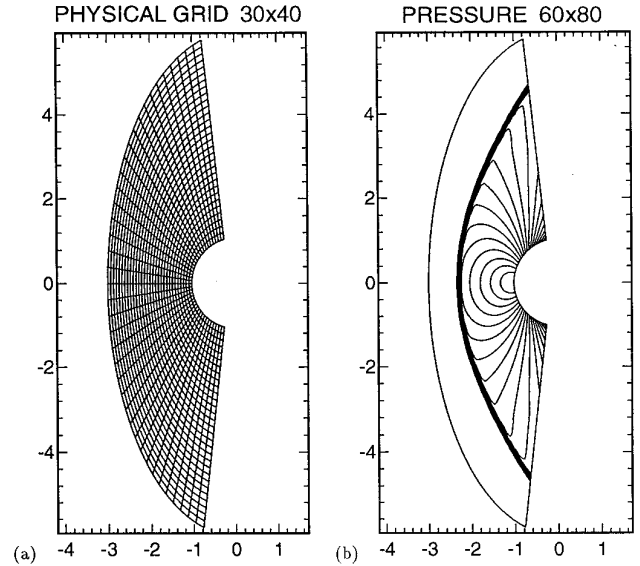
FIG. 16. Flow past a cylinder: (a) physical grid; (b) pressure. WENO-LF-5 with RK-4, 20 contours.
