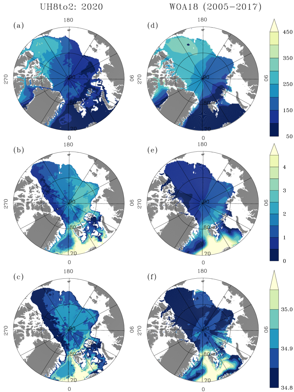
Figure 9: Atlantic layer characteristics in the UH8to2 (year 2020) and WOA18 (data from 2005-2017). Top: depth (m), defined as the upper-most depth in the water column below 50 m of the 0^{\circ}\text{C} isotherm for a) UH8to2 (2020) and d) WOA18. Middle: maximum temperature ( ^{\circ}\text{C} ) in the Atlantic layer located between the subsurface 0^{\circ}\text{C} isotherms where salinities are greater than 34.8 for b) UH8to2 and e) WOA18. Bottom: salinity ( \text{g kg}^{-1} ) at the depth of the temperature maximum from c) UH8to2 and f) WOA18.
