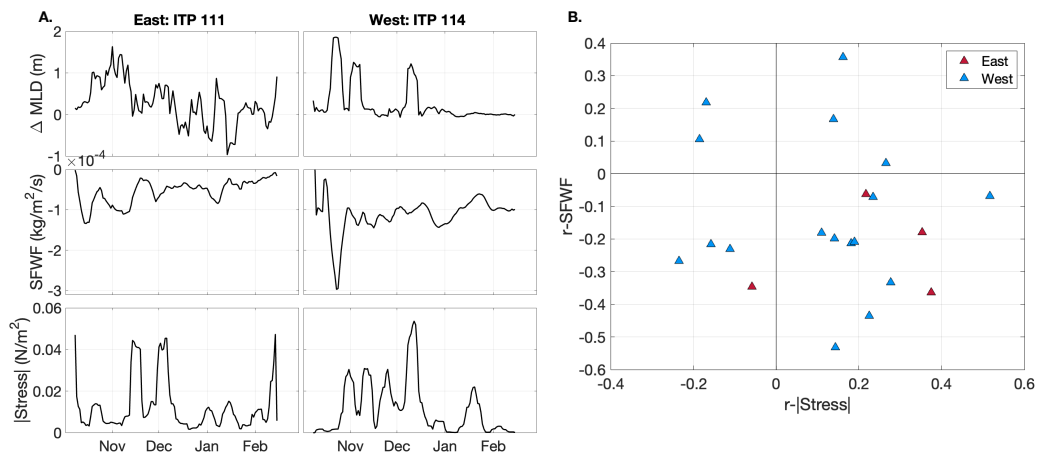
Figure 17: A. 7-day smoothed time series of the change in mixed layer depth (m; top), net surface freshwater flux ( \text{kg m}^{-2} \text{s}^{-1} ; middle), and ice-ocean stress magnitude ( \text{N m}^{-2} ; bottom) in the eastern (left) and western (right) example ITP deployments. All quantities are for the synthetic UH8to2 ITP deployments. B. Partial correlations of the winter change in mixed layer depth with net surface freshwater flux and ice-ocean stress magnitude for each synthetic ITP deployment that had at least 20 profiles between October and March of the following year. Partial correlations are calculated from the 7-day smoothed time series.
