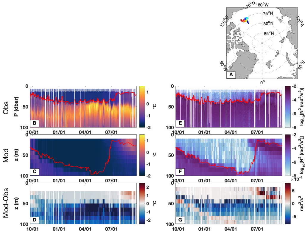
Figure 15: ITP #114 section in the western Arctic (as in fig. 14). a) Overhead map of ITP deployment, b) observed temperature ( ^{\circ}\text{C} ), c) modeled temperature along deployment ( ^{\circ}\text{C} ), d) model-observed temperature difference ( ^{\circ}\text{C} ), e) observed buoyancy frequency ( \text{rad}^2 \text{s}^{-2} ), f) modeled buoyancy frequency ( \text{rad}^2 \text{s}^{-2} ), g) model-observed buoyancy frequency difference ( \text{rad}^2 \text{s}^{-2} ). The mixed layer depth is shown as a red line in panels b,c,e, and f.
