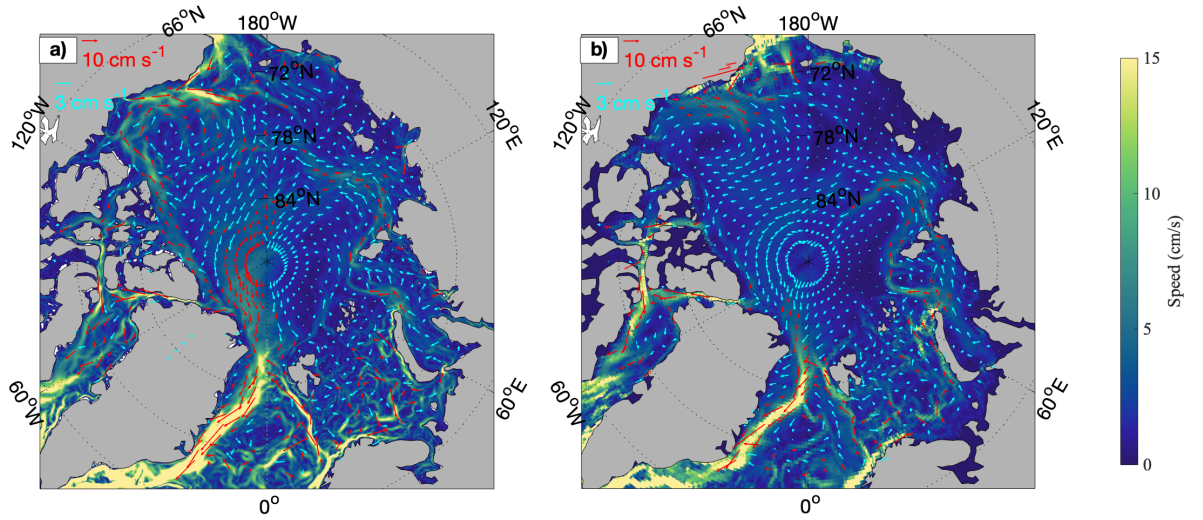
Figure 4: 2017 Arctic surface velocities ( \text{cm s}^{-1} ) from a) the UH8to2 model and b) the ASTE estimate (Nguyen et al., 2021). The ASTE estimate was interpolated onto a 0.3 degree grid in latitude and longitude for this comparison.
