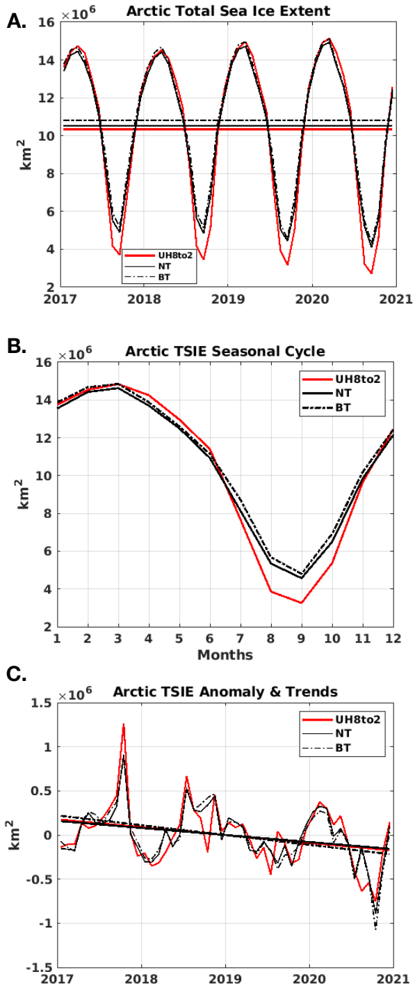
Figure 5: a) Monthly total sea ice extent (TSIE, sum of the sea-ice area in which sea-ice concentration is greater or equal to 15%, units of \text{km}^2 ) from the UH8to2 simulation, satellite observations using the NASA Team (NT) algorithm, and bootstrap algorithm (BT); b) seasonal cycle of TSIE averaged over the 2017-2020 UH8to2 run; c) TSIE seasonal anomaly and trend over 2017-2020.
