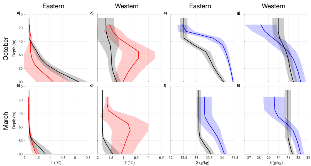
Figure 16: a)-d) Mean temperature ( ^{\circ}\text{C} ) profiles in the upper ocean, for the months of October (a and c) and March (b and d) for the Eastern (a and b) and Western (c and d) Arctic; e)-h) Mean salinity ( \text{g kg}^{-1} ) profiles in the upper ocean, for the months of October (e and g) and March (f and h) for the Eastern (e and f) and Western (g and h) Arctic. Colored profiles represent ITP observations, while black profiles are averages from the UH8to2 model. The shaded regions represent two standard deviations around the mean.
