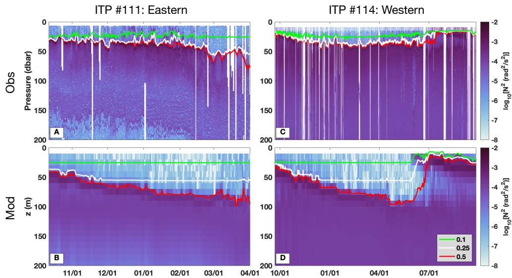
Figure 3: Stratification ( \text{rad}^2 \text{s}^{-2} ) and mixed layer depths over two example ITP deployments as follows: a) ITP 111 (eastern Arctic), observed; b) ITP 111 (eastern Arctic), modeled; c) ITP 114 (western Arctic), observed; and d) ITP 114 (western Arctic), modeled. The three lines represent mixed layer depths calculated using a threshold difference in \delta\sigma of 0.1 (green), 0.25 (white), and 0.5 (red) \text{kg m}^{-3} . Throughout the rest of the study, \delta\sigma = 0.5 \text{ kg m}^{-3} is used to define the mixed layer depth, as this value agreed best with the evolution of the deepening peak in N^2 through the winter, especially in the model fields
