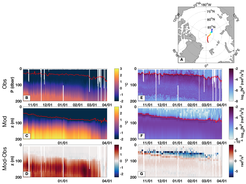
Figure 14: ITP #111 section in the eastern Arctic. a) Overhead map of ITP deployment, b) observed temperature ( ^{\circ}\text{C} ), c) modeled temperature ( ^{\circ}\text{C} ) along ITP deployment, d) model-observed temperature difference ( ^{\circ}\text{C} ), e) observed buoyancy frequency ( \text{rad}^2 \text{s}^{-2} ), f) modeled buoyancy frequency ( \text{rad}^2 \text{s}^{-2} ), g) model-observed buoyancy frequency difference ( \text{rad}^2 \text{s}^{-2} ). The mixed layer depth is shown as a red line in panels b,c,e, and f.
