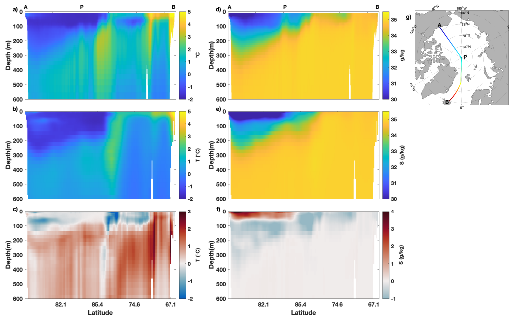
Figure 8: Cross-Arctic sections of a) four-year average UH8to2 temperature ( ^{\circ}\text{C} ), b) WOA18 (2005-2017) temperature ( ^{\circ}\text{C} ), c) four-year average UH8to2 and WOA18 (2005-2017) temperature difference ( ^{\circ}\text{C} ), d) four-year average UH8to2 salinity ( \text{g kg}^{-1} ), e) WOA18 (2005-2017) salinity ( \text{g kg}^{-1} ), and f) four-year average UH8to2 and WOA18 (2005-2017) salinity difference ( \text{g kg}^{-1} ), with g) overhead view of the cross-Arctic section. Panels a) through f) are oriented so that the western Arctic (north of Canada) is on the left hand side of the panel.
