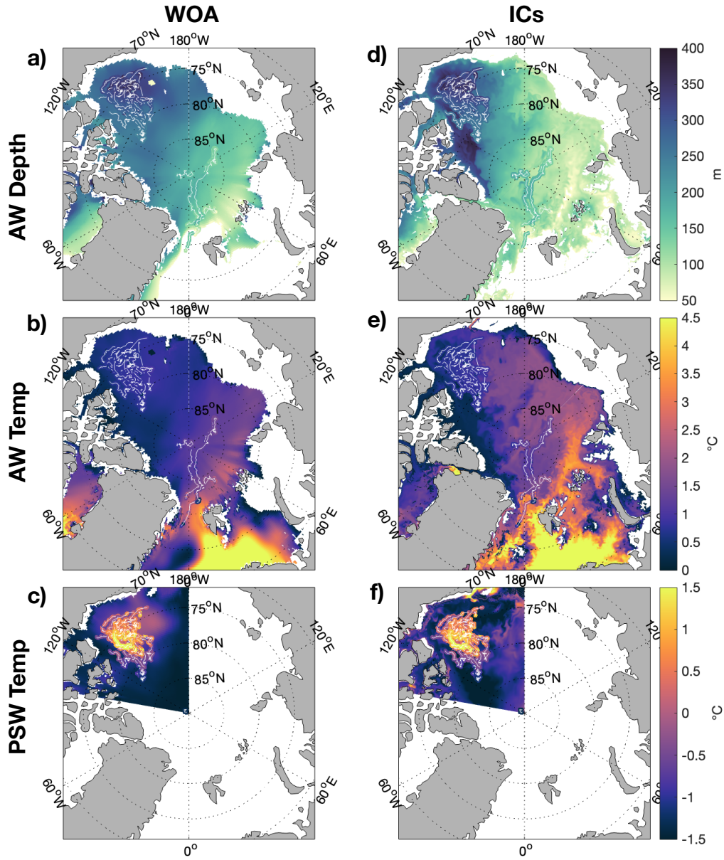
Figure 2: Comparisons between the WOA18 (2005-2017) climatology (a,b,c), UH8to2 initial conditions (d,e,f), and ITP profiles from 2017-2020 of (top) Atlantic Water Depth (m), (middle) Atlantic Water Temperature (°C), and (bottom) Pacific Summer Water temperature (°C)
