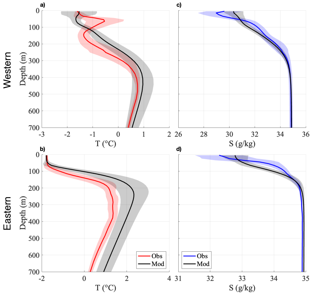
Figure 11: Comparison of mean ITP-observed profiles (red and blue) and matched synoptic model profiles (black) of a) temperature ( ^{\circ}\text{C} ) in the western Arctic (latitudes between 0 and 180^{\circ}\text{W} ), b) temperature ( ^{\circ}\text{C} ) in the eastern Arctic (latitudes between 0 and 180^{\circ}\text{E} ), c) salinity ( \text{g kg}^{-1} ) in the western Arctic (latitudes between 0 and 180^{\circ}\text{W} ), and d) salinity ( \text{g kg}^{-1} ) in the eastern Arctic (latitudes between 0 and 180^{\circ}\text{E} ). Shaded regions represent a standard deviation around the mean. In total the ITP record includes 4218 profiles in the east and 35724 profiles in the west.
