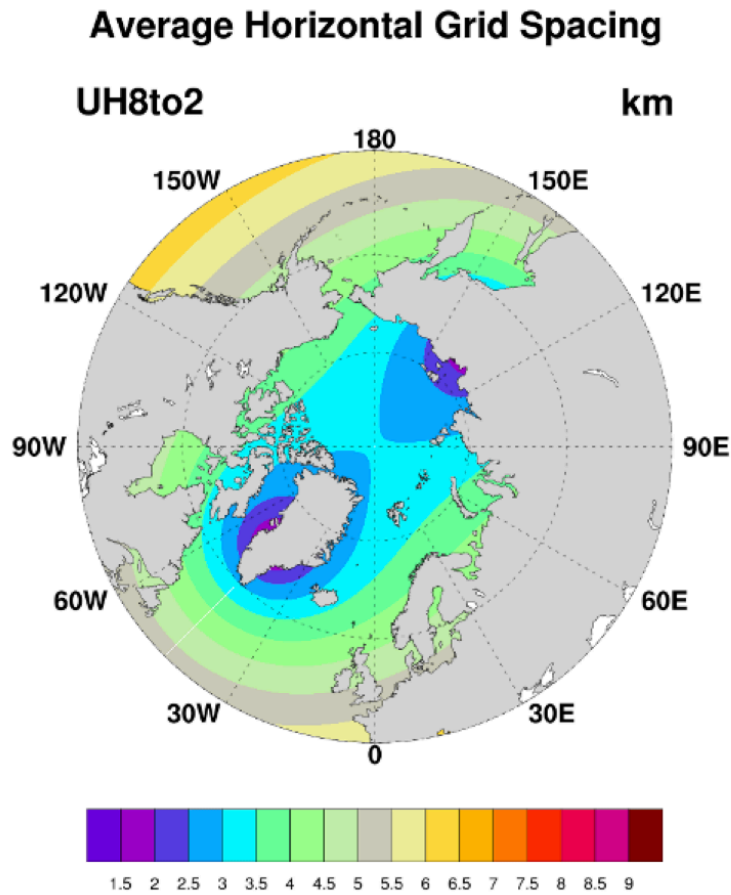
Figure 1: Square root of horizontal area (km) of grid cells in the Arctic region of the UH8to2 POP model.
