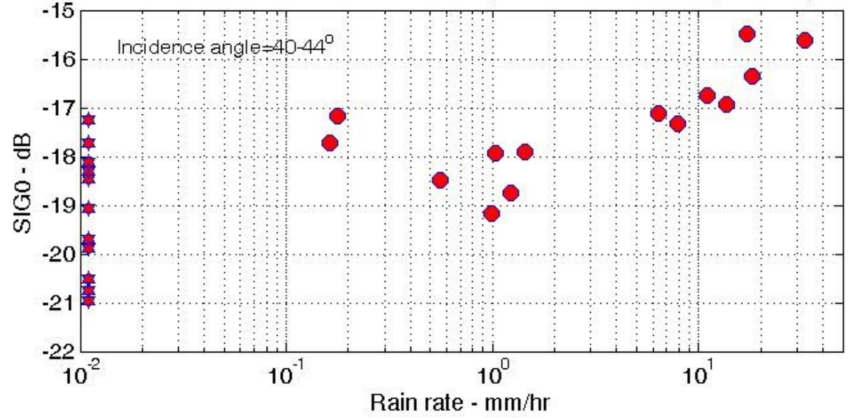
ASCAT - NRCS vs Rain Rate, Aft Beam, Sequence of Incidence Angles, 19-Apr-09
