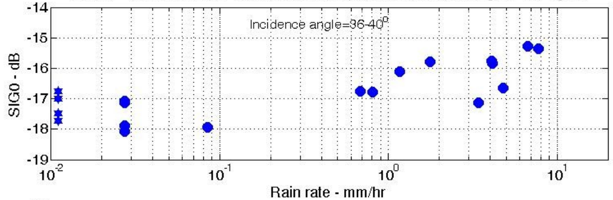
ASCAT - NRCS vs Rain Rate, Aft Beam, Sequence of Incidence Angles, 13-Aug-08
