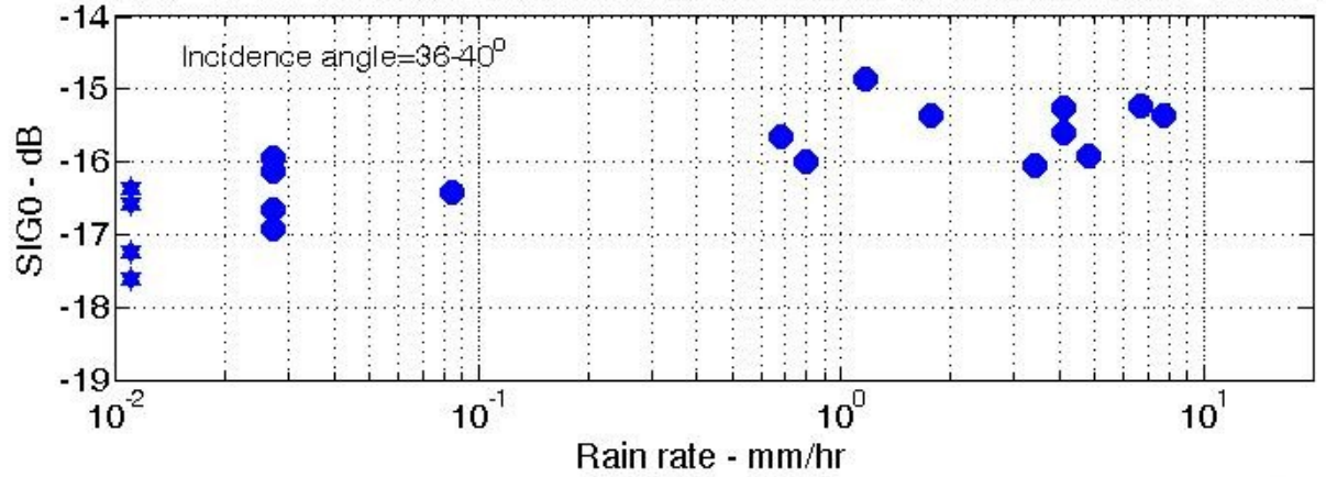
ASCAT - NRCS vs Rain Rate, Forward Beam, Sequence of Incidence Angles, 13-Aug-08
