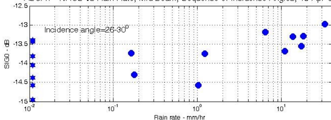
ASCAT - NRCS vs Rain Rate, Mid Beam, Sequence of Incidence Angles, 19-Apr-09
