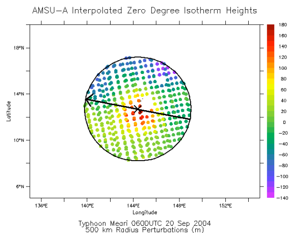
Figure 4. Perturbation freezing level heights in meters for a 500 km radius (black ellipse) at the time indicated in the figure. Storm center indicated by an "X" with the arrow representing the storm motion vector. Colored circles mark the centers of the elliptical footprints from the AMSU-A
