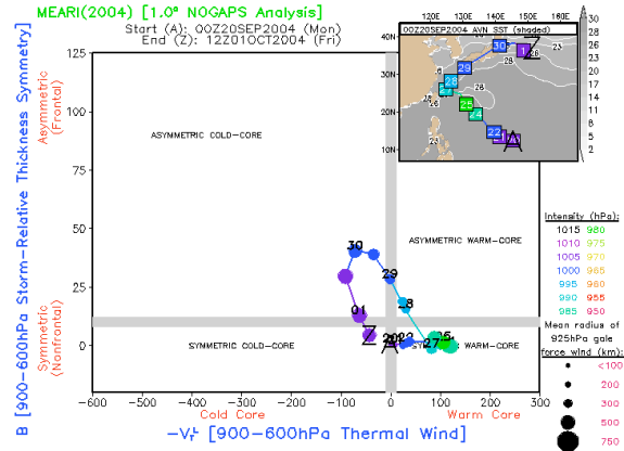
Figure 7. Cyclone Phase Space (CPS) diagram for Typhoon Meari using 1° NOGAPS analyses every 12 h. Details of plot are labeled on the diagram. Courtesy of Dr. Robert Hart ( http://moe.met.fsu.edu/cyclonephase/index.html )
