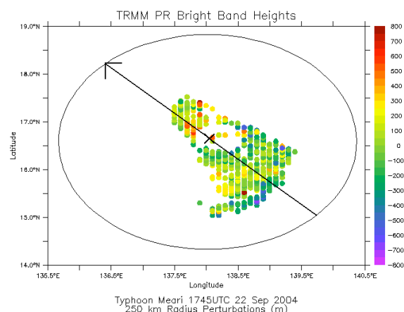
Figure 2. Perturbation freezing level heights in meters for a 250 km radius (black ellipse) at the time indicated in the figure. Storm center indicated by an “X” with the arrow representing the storm motion vector. Colored circles mark the centers of the elliptical footprints from the TRMM PR.
