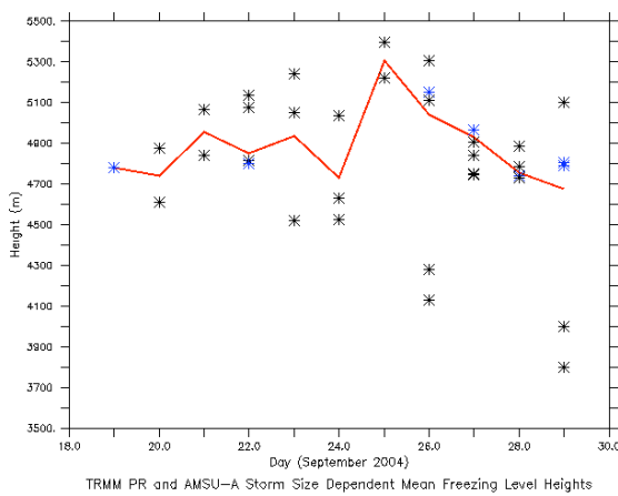
Figure 6. Time series plot of freezing level heights synthesizing data from the TRMM PR and AMSU-A for the life cycle of Typhoon Meari. Blue stars mark TRMM PR data while black stars represent the AMSU-A. The red line shows the weighted mean fit to the data.
