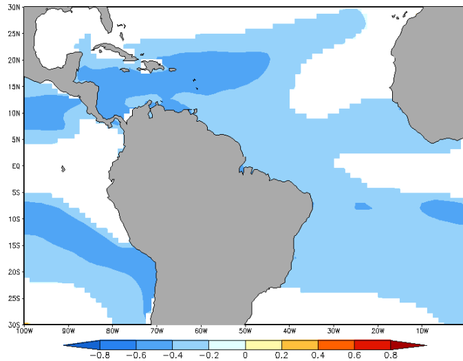
Fig. 2: Correlation of DJF seasonally averaged rainfall over the boxed region ( 50^{\circ}\text{W} - 65^{\circ}\text{W} and 7^{\circ}\text{S} - 7^{\circ}\text{N} ) with the following JJA seasonally averaged SST from the CESM1.0 control integration. Only correlation at 10% significance level according to t-test is shown. The period of data used here is from 1901-2000.
