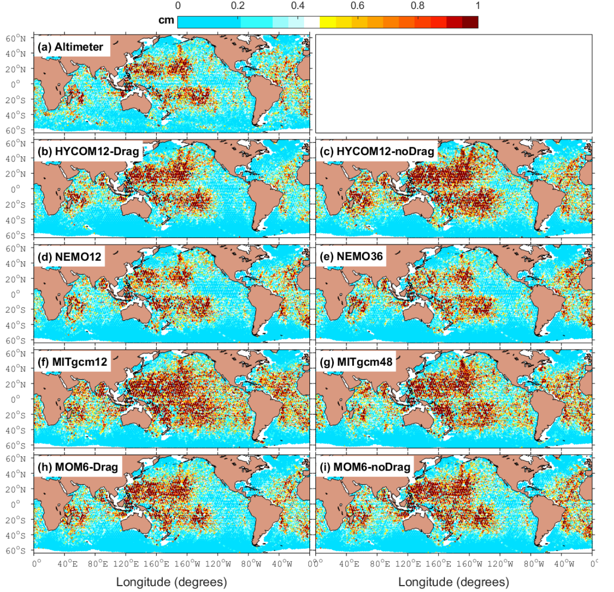
Figure 4. Amplitude (cm) of M_2 internal tides in (a) along-track altimeter-based analyses, and in (b) HYCOM (Experiment E051, with wave drag), (c) HYCOM (Experiment E053, no wave drag), (d) NEMO12, (e) NEMO36, (f) MITgcm12, (g) MITgcm48, (h) MOM6-Drag, (i) MOM6-noDrag. The amplitudes of the MITgcm12 simulation are computed from 6 months of SSH output, while all others are based on 12 months of output.
