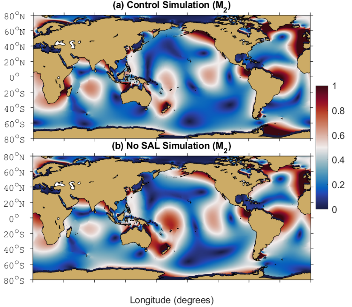
Figure 2. (a) Amplitudes of the M_2 surface elevations, from the shallow-water barotropic tide model of Schindelegger et al. (2018). (b) Same as in (a) but without the SAL term in the momentum equation, and with an astronomical tidal forcing that is increased by a factor of 1.1121, in order to mimic the forcing of the MITgcm simulations shown here.
