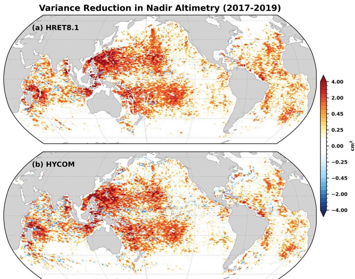
FIG. 9. Global maps of internal tide SSH variance reduction in nadir altimetry by (a) the empirical HRET8.1 model and (b) 1/25° HYCOM forecasts. The HYCOM results come from a 3-yr harmonic analysis of total SSH after applying a Gaussian spatial filter to extract the coherent internal tide signal. Adapted from Yadidya et al. (2024).
