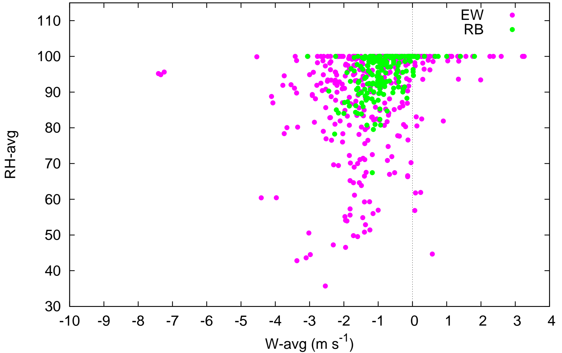
CAT 345 DOWN W-avg vs RH-avg EW/RB N=570
