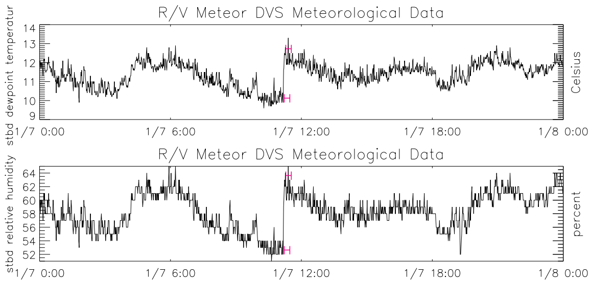
Figure 3: Moisture discontinuity
