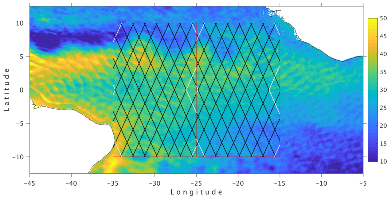
Figure 9. Topex/Poseidon (T/P) tracks in four 10 \times 10^\circ boxes in the equatorial Atlantic. The color shading displays a snapshot of the modeled steric SSH (in cm) from NEATL-T-HB-HF. The black lines denote the nominal and interlaced T/P tracks in each box that are longer than 500 km and used for wavenumber spectra calculation; the white lines are the track segments that are shorter than 500 km and not used.
