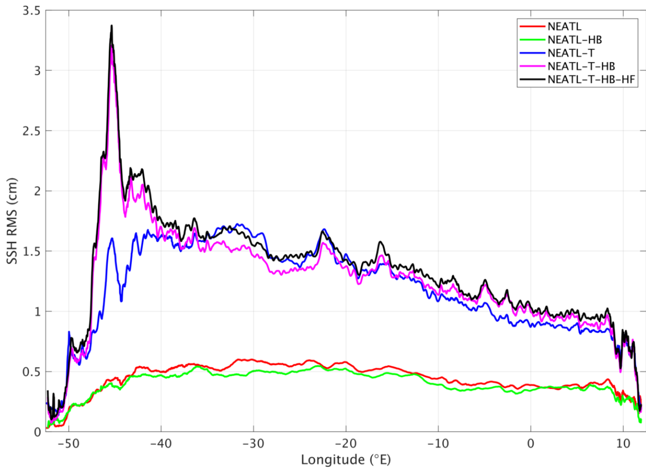
Figure 3. Standard deviation of the high-frequency steric sea surface height (SSH, in cm) variability in the equatorial Atlantic (averaged between 5°S and 5°N) in five 1/50° Atlantic simulations that are shown in Figure 2: a) NEATL, b) NEATL-HB, c) NEATL-T, d) NEATL-T-HB, and e) NEATL-T-HB-HF.
