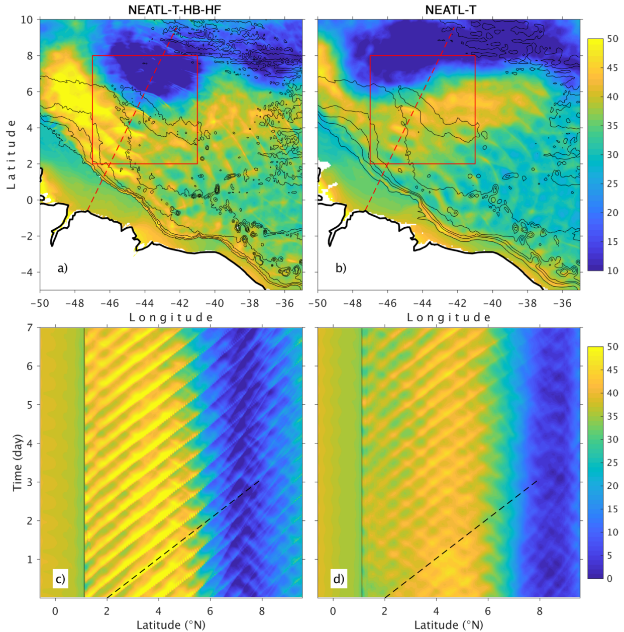
745 Figure 4. Internal tide generation off the Amazon shelf in two simulations with and without high- resolution bathymetry: NEATL-T-HB-HF (a & c), NEATL-T (b & d). Panels a-b show a snapshot of the steric SSH (in cm); panels c-d show a Hovmöller diagram of the steric SSH (in cm) along the dashed red line in panels a-b. Black solid line indicates the location of shelf break at 100-m isobath (see also the insert panel in Figure 6b) and black dashed line indicates a northward phase speed of 2.5 m/s.
