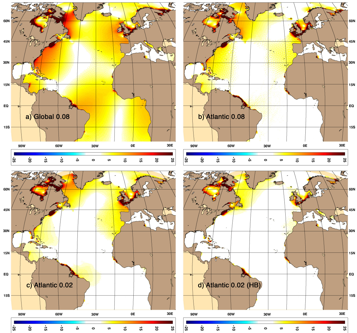
720 Figure 1. Root-square-mean (RMS) error in cm of the modeled barotropic M_2 tide in four HYCOM simulations compared to TPX08: a) 1/12^\circ Global simulation; b) 1/12^\circ Atlantic simulation; c) 1/50^\circ Atlantic simulation NEATL-T (with bathymetry interpolated from 1/12^\circ simulation); and d) 1/50^\circ Atlantic NEATL-T-HB (with bathymetry calculated from 30 arc-sec GEBCO_2019).
