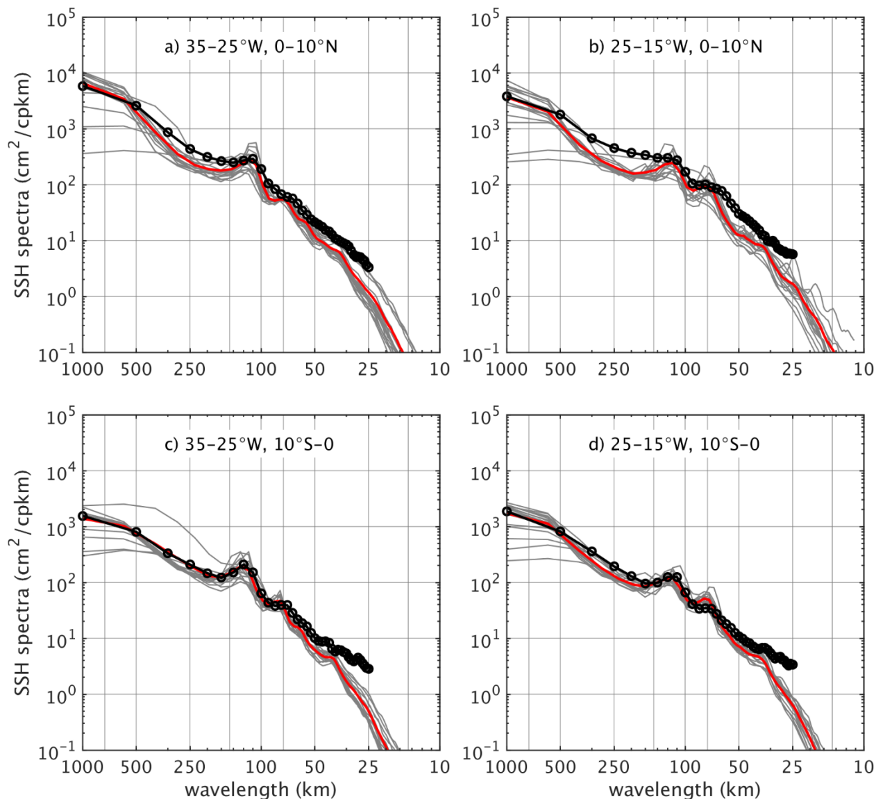
805 Figure 10. SSH wavenumber spectra calculated from T/P tracks in four 10 \times 10^\circ boxes in the equatorial Atlantic. The gray curves are modeled (NEATL-T-HB-HF) wavenumber spectra based on individual tracks and the red curves are their average, representing the modeled wavenumber spectra of the box. The circled black curves are the observation results from Zhou et al. (2015).
