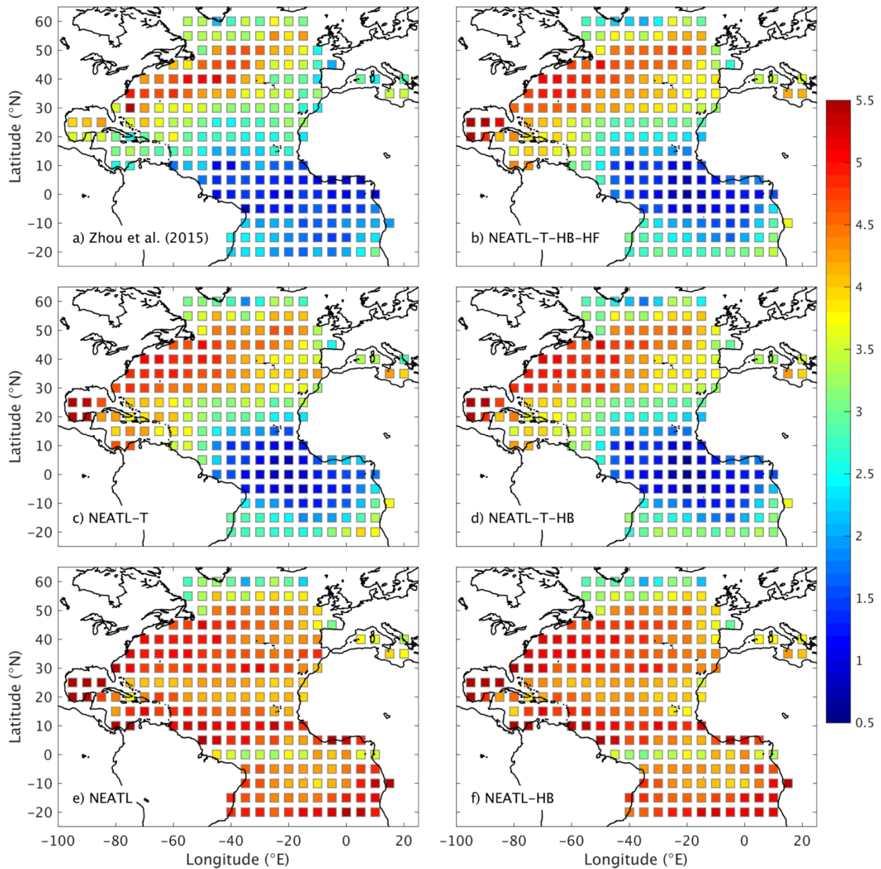
Figure 7. Slope of SSH wavenumber spectra in the Atlantic Ocean from observations (Zhou et al. 2015) and five Atlantic simulations. The slope is for mesoscale range (70-250 km) and the value is inverted (multiplied by -1).
