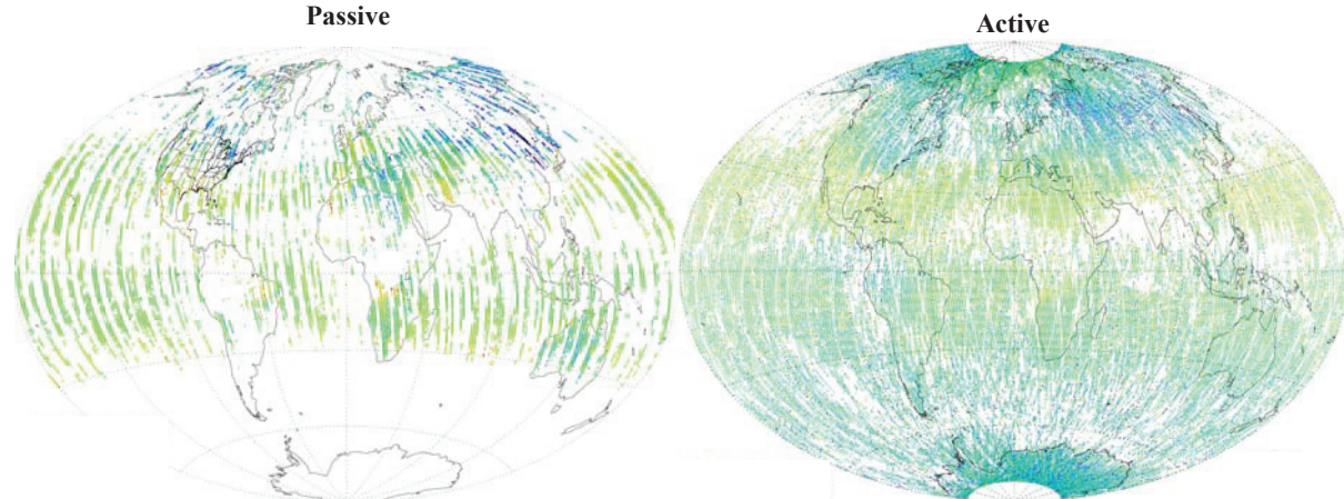
Figure 7.8. Spatial coverage of (left) passive and (right) active instruments in July. Reasons for gaps in passive coverage include low light (southern hemisphere in this image), high particulate matter levels and clouds (e.g., polar regions and areas experiencing monsoons). [Image courtesy of Randy Kawa (NASA).]
