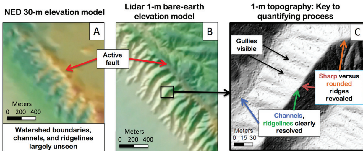
FIGURE 10.17 (A) A shaded-relief image of a portion of the Dragon's Back Pressure Ridge derived from the 30-m-resolution National Elevation Dataset (NED) fails to resolve basic landscape attributes, such as watershed boundaries, ridgelines, and channels. SOURCE: Dataset from the USGS. (B) High resolution (1 m) bare-earth topography of the same area clearly shows the location of the active San Andreas Fault and discriminates fundamental landscape elements. SOURCE: Data from www.opentopography.org . (C) A close-up clearly reveals the transition between gullies, hillslopes, and channels, as well as changes in the geometry of these landforms that result from variations in the rates of surface processes and fault-related uplift. SOURCE: Modified from Hurst et al. (2013).
