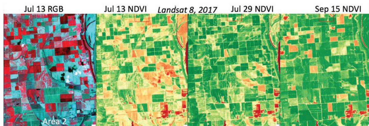
Figure 8.7. Landsat-8 Operational Land Imager images of Central Arkansas from July 13, July 29, and September 15, 2017. These images show the 30 m multi-spectral monitoring potential of Landsat-8 where individual fields can be discriminated and crop type determined from multi-temporal acquisitions during the growing season. SOURCE: Landsat-8 Project Office, NASA/Goddard Space Flight Center.
