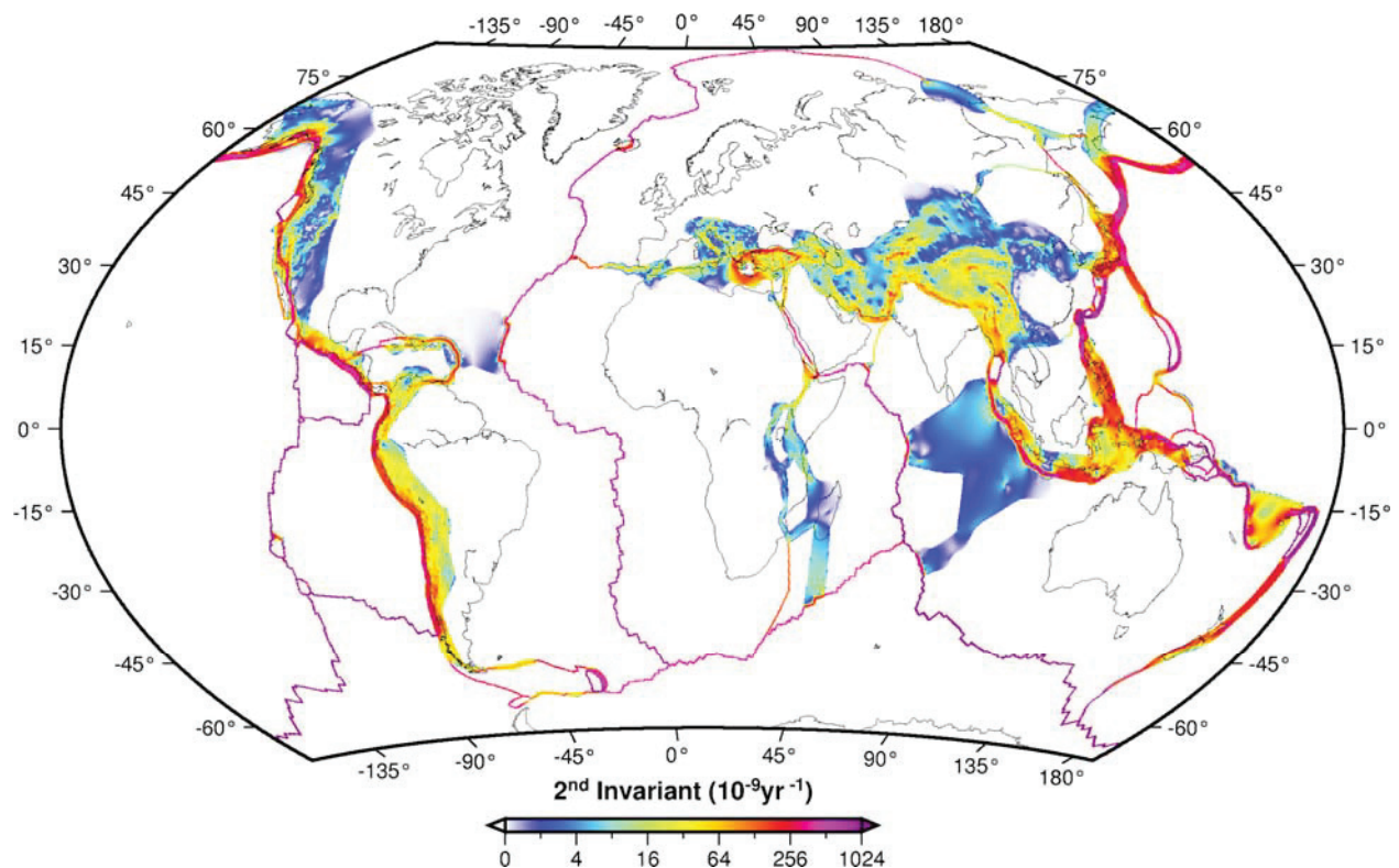
FIGURE 10.21 Color contours of the strain rate along the boundaries of the major tectonic plates derived from 22,500 GPS velocities. Most major earthquakes occur in these high strain rate areas, and so refined mapping is needed to improve the accuracy of the global earthquake hazard maps as well as to better understand the physics of plate boundaries as well as the extent and physics of intraplate deformation. SOURCE: Kreemer et al. (2014).
