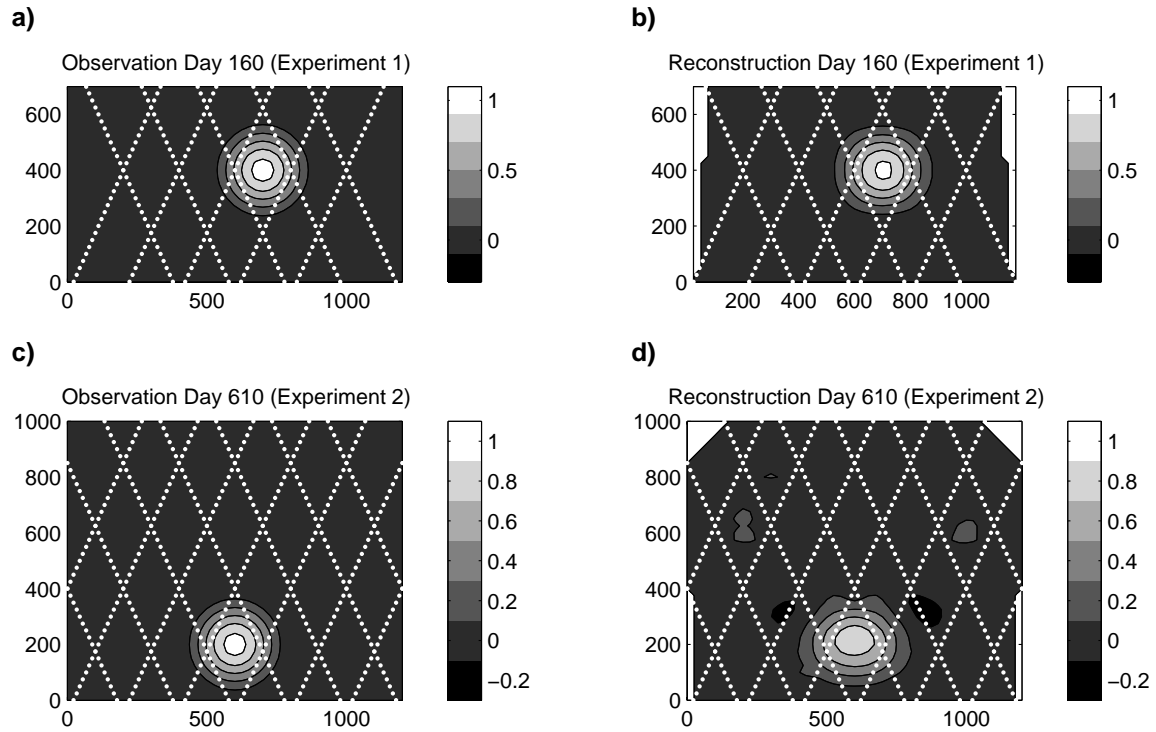
Figure 2. a) The synthetic SSH field for Experiment One with an eddy moving westward; b) The reconstructed field for Experiment One; c) The synthetic SSH field for Experiment Two with an eddy moving anticlockwise around the center of the domain; d) The reconstructed field for Experiment Two. The white dots are simulated satellite tracks.
