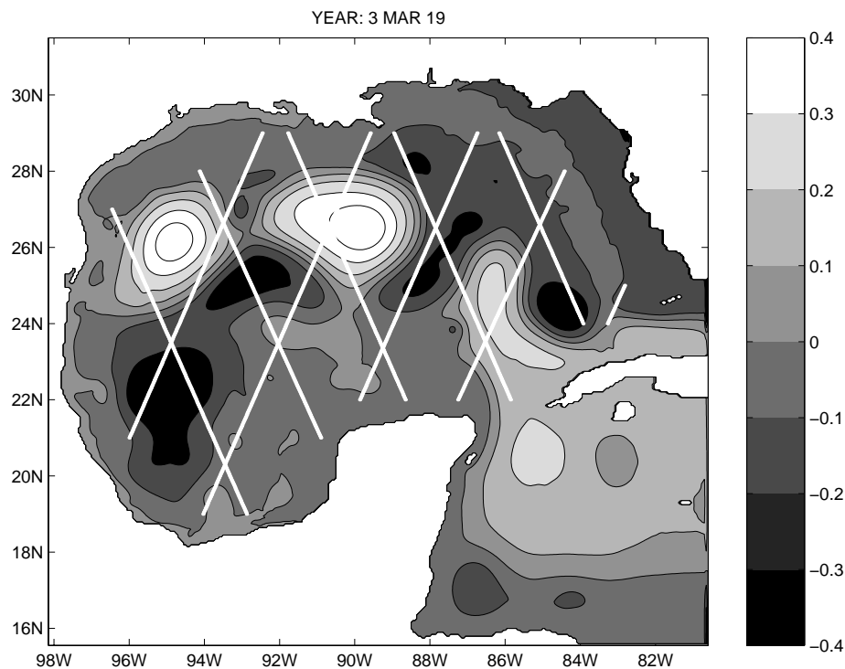
Figure 1. The sea surface height from the COAPS/FSU Gulf of Mexico numerical simulation using the Navy Coastal Ocean Model (NCOM). The white lines are simulated Topex/Poseidon tracks.
